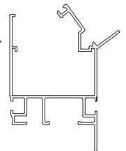
Gutter profile
