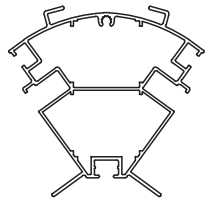
Ridge Beam Profile
